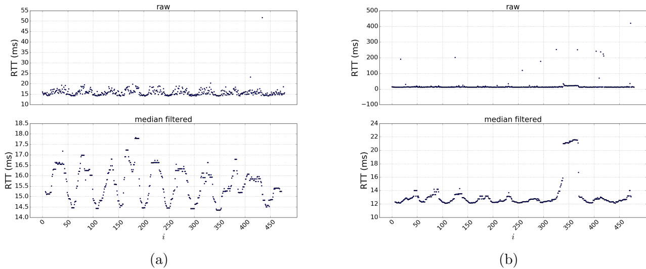
Figure 3.1: Median filter RTT. w = 6 . Plots with different scales.
