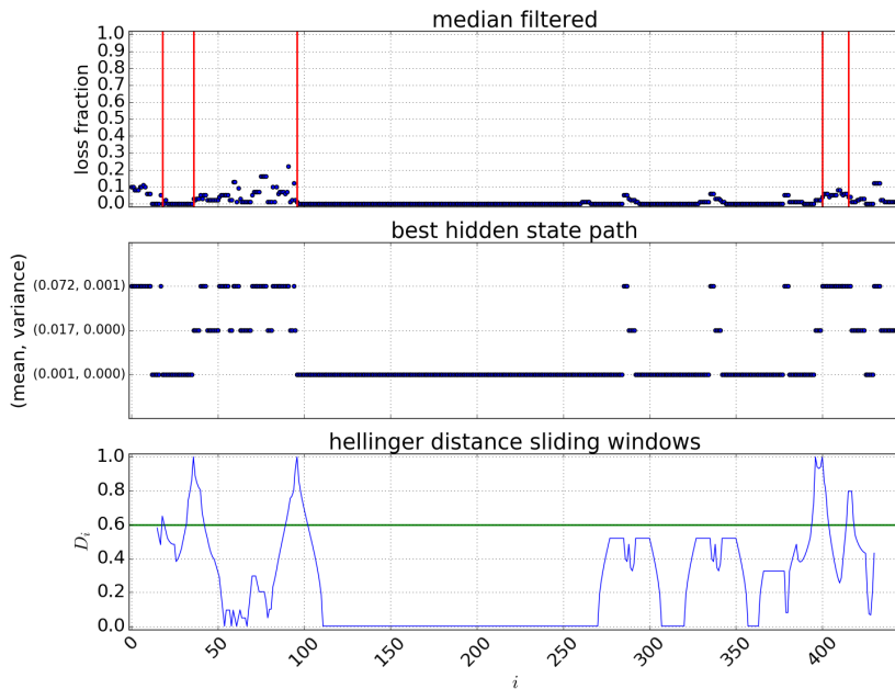
Figure 3.6: HMM filter.
